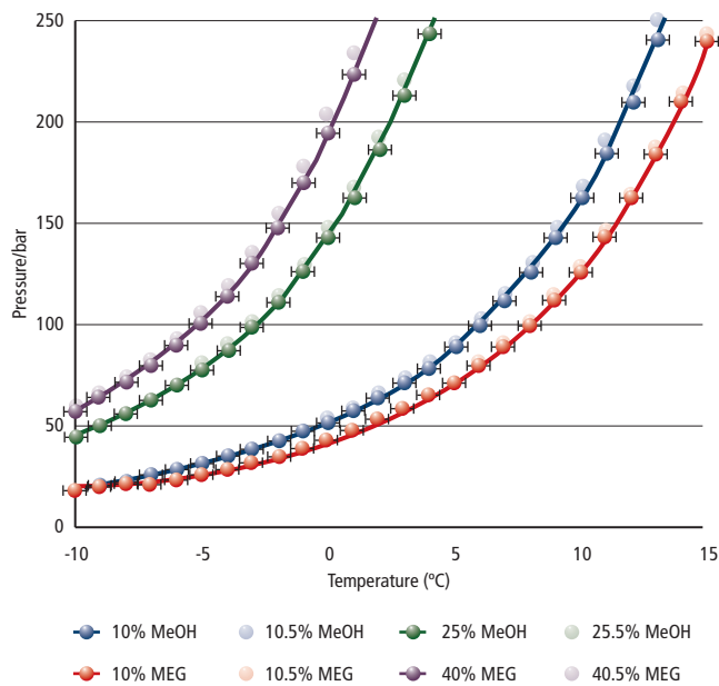
Figure 2: Possible Shifts in Methane Hydrate Phase Boundaries Owing to the Maximum Measurement Errors of the Prototype C-V Device
