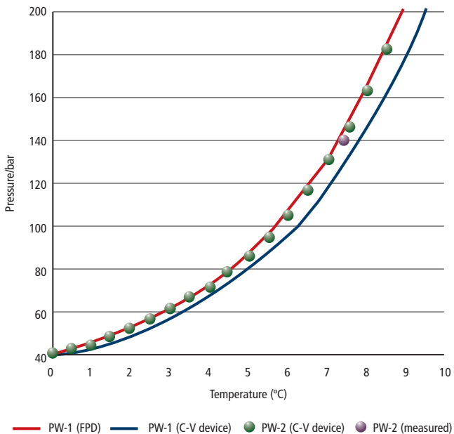
Figure 3: Evaluation of the Prototype C-V Device Using Two Real Produced Water Samples Containing Unknown Concentrations of Methanol, a Corrosion Inhibitor and Multi-component Salts in Addition to the Presence of Condensate
