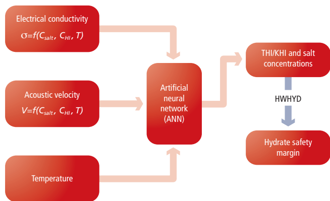
Figure 1: Methodological Chart of the Hydrate Inhibition Monitoring System
